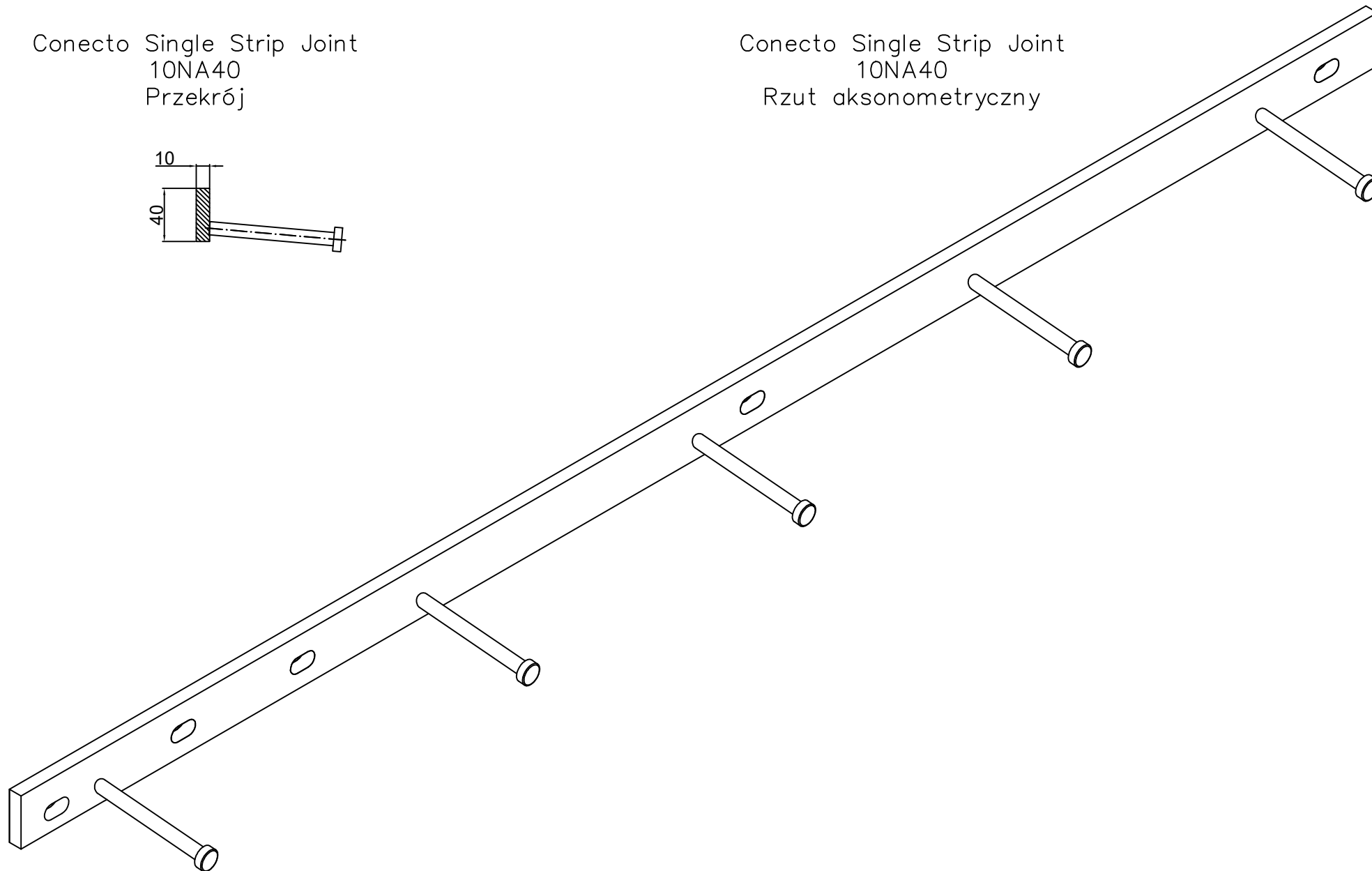
Conecto Single Strip Joint 10NA40 stal ocynkowana (PC)
