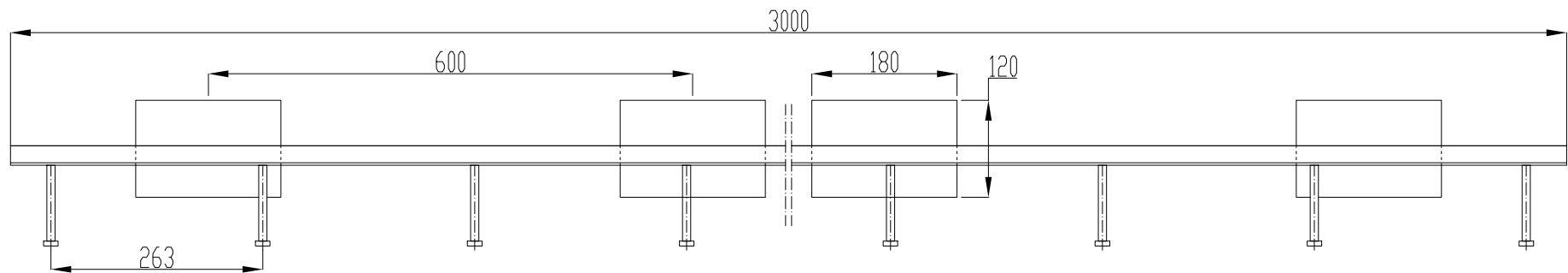
Conecto Omega 03NB-5D-T8 h=140/155 Top view scale 1:1,25
